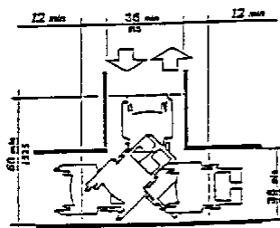
(b) T-Shaped Space for 180° Turns
