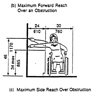
Fig. 2 Reach Ranges
