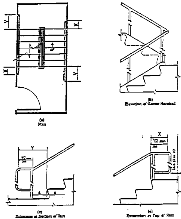
Fig. 18 Usable Tread Width and Examples of Acceptable Nosings
