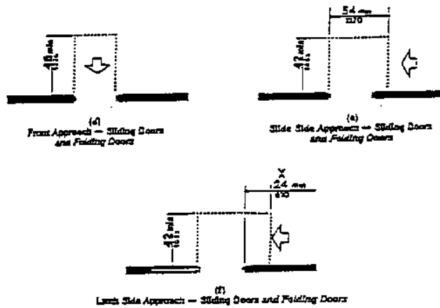
Fig. 25 Maneuvering Clearances at Doors (Continued)
