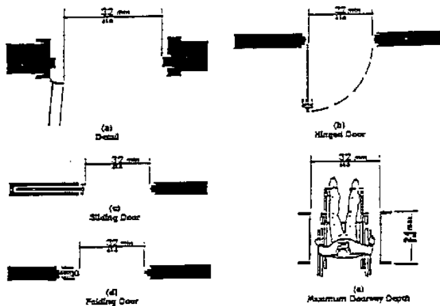
Fig. 24 Car Doorway Width and Depth
