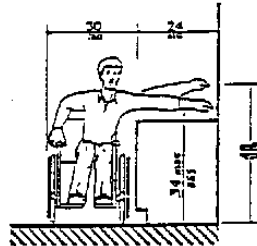
Maximum Side Reach over Obstruction
