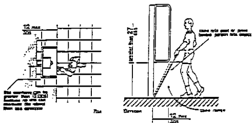
Fig. 3 Protruding Objects (Continued)
