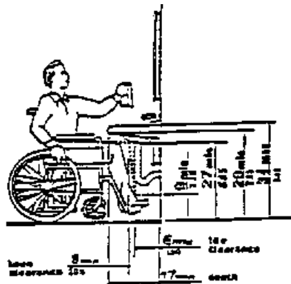
Fig. 31 Livery Clearance
